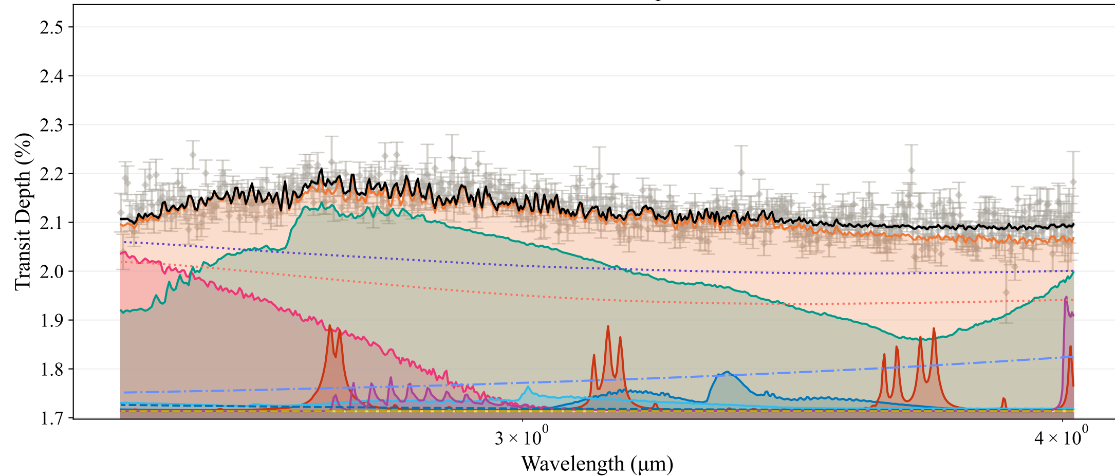
NIRCAM, SiO, 4-point
